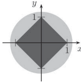
Fig. 2. \{|x| + |y| < 1\} (dark gray) and D(0, R_0) (light gray).
