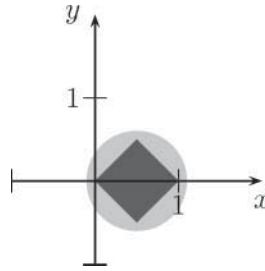
Fig. 1. \left\{ \left| x - \frac{1}{2} \right| + |y| < \frac{1}{2} \right\} (dark gray) and D(z_0, R_0/2) (light gray).
